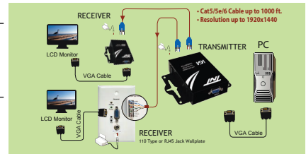
Receiver R02T-EXT-C5E-RMT Receiver R02T-EXT-RX-FP Receiver R02T-EXT-C5E-RMT 1U 19" Rack Mountable Panel R02-SPL-PANEL
