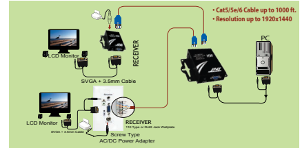
Receiver R02T-EXT-C5E-35A-RMT Receiver R02T-EXT-35A-RX-FP Receiver R02T-EXT-35A-RX-JP 1U 19" Rack Mountable Panel for 1x4 Splitter R02-SPL-PANEL
